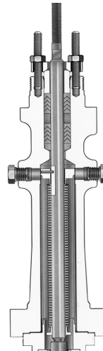
Figure 1-6. Bellows Seal Bonnet
