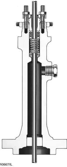
Figure 6-3. Typical Extension Bonnet
