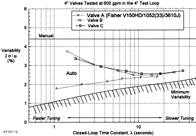
Figure 2-7. Closed-Loop Performance
