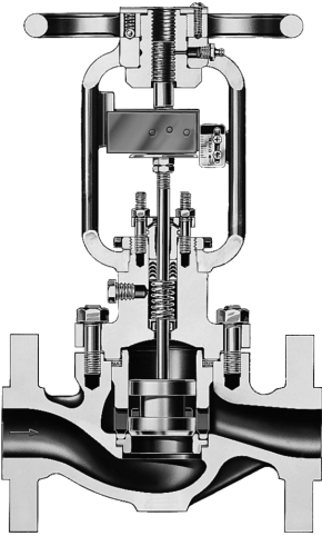
Figure 3-37. Typical Manual Actuators
