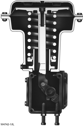
Figure 3-34. Diaphragm Actuator for Rotary Shaft Valves
