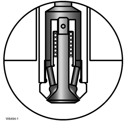
Figure 7-10. Variable Geometry, Backpressure Activated Spray Nozzle
