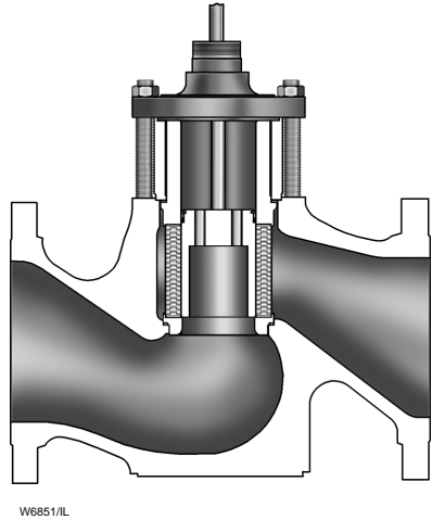
Figure 5-13. Globe Style Valve with Noise Abatement Cage for Aerodynamic Flow
