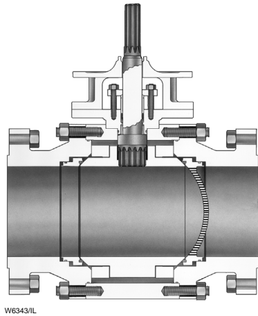
Figure 5-14. Ball Style Valve with Attenuator to Reduce Hydrodynamic Noise
