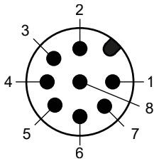
M12 Circular connector, 8 pin (setpoint)
