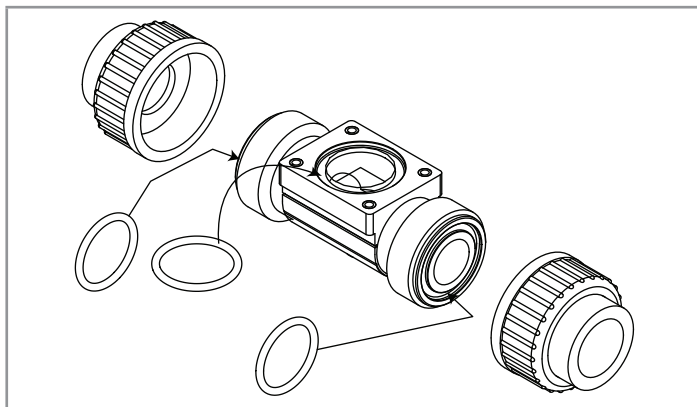
Fig. 14: Seals for plastic fitting
