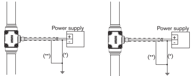
8011 with cable gland
