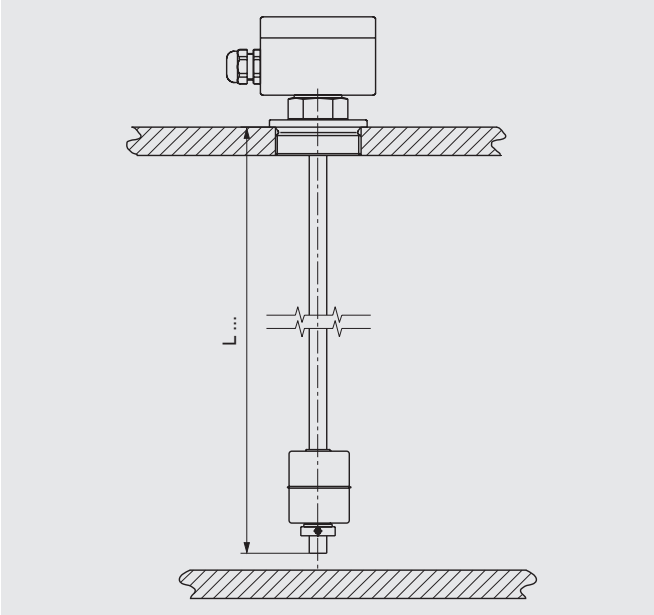
Version A: Fixed to the tank ceiling
