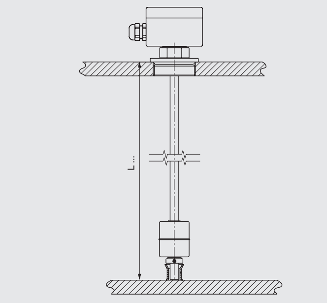
Version B: Fixed to the tank ceiling and floor
