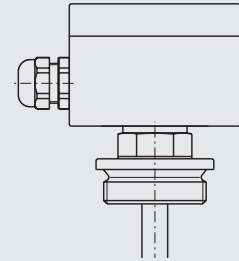
Mounting thread and connection housing
